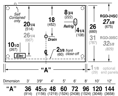
RGD 24, 30 Remote and Self Contained plan view
